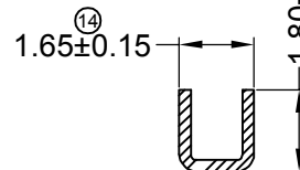
SECTION C-C SCALE 1:1
