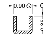
SECTION C-C SCALE 1 : 1
